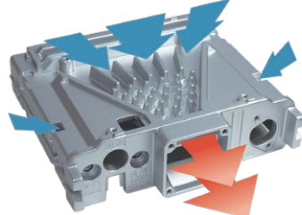
FACC: Funnel Air-Convection Conductor (Wind Tunnel)
